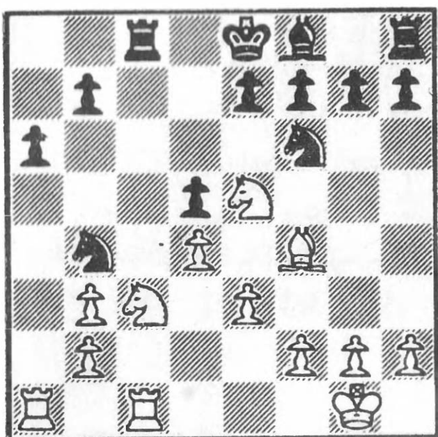
83 After 14...Ke8
